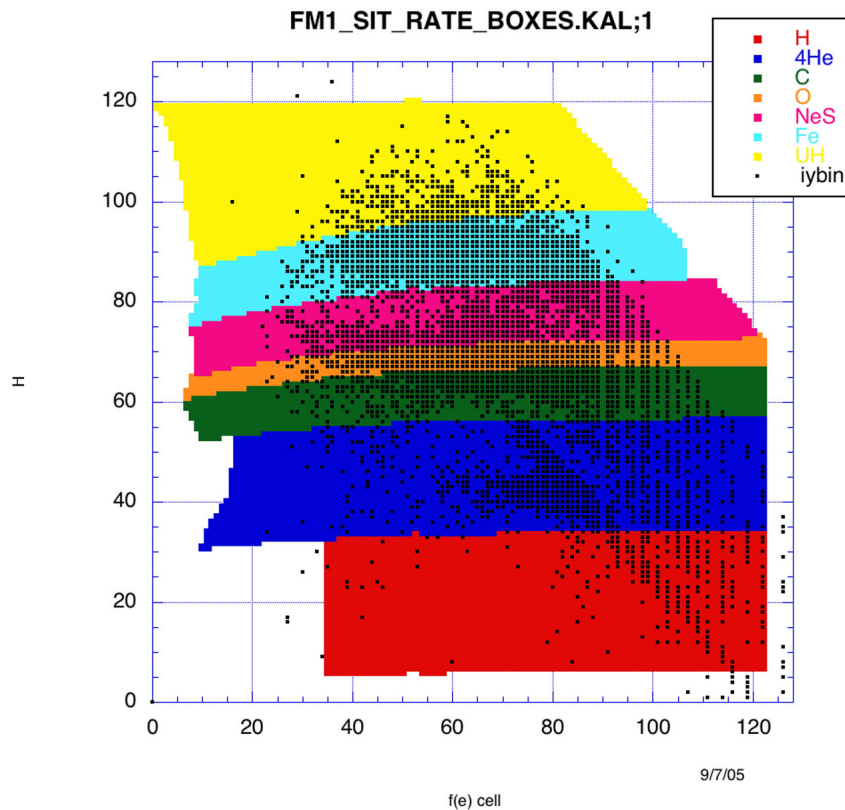
Figure 3. Valid Events (black dots from fm1 BNL calibration, August 2004) superposed on fm1 rate bin grid (v. 090105). Different elements have different colors; within each element are a number of
