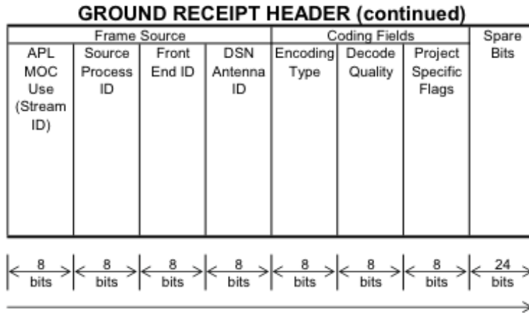
Figure 16. Ground Receipt Header Data Structure Diagram (2 of 2)
