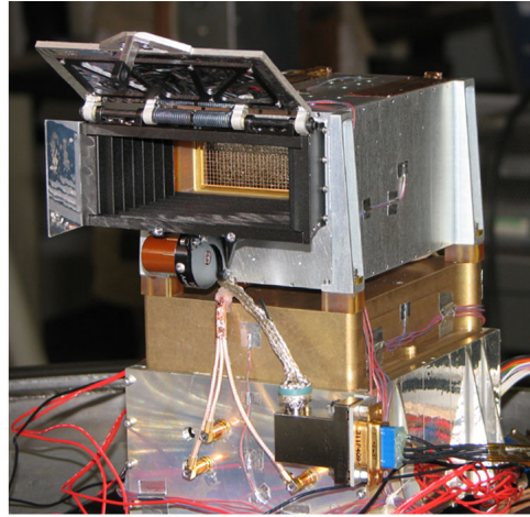
SIT - Suprathermal Ion Telescope
